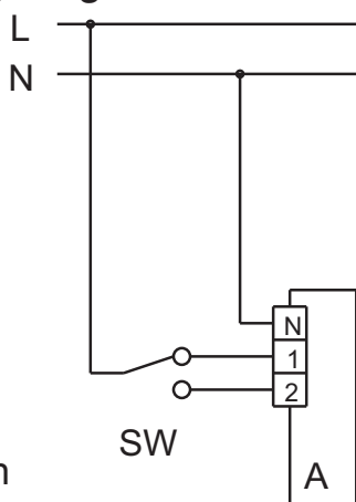
wiring diagram 5
