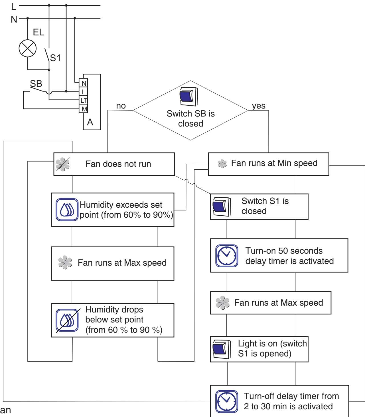
wiring diagram 10
